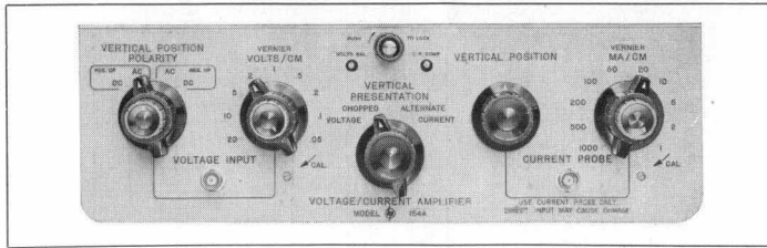
Fig. 10. Panel view of hp-Model 154A Voltage/Current Plug-in Amplifier .
