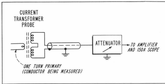
Fig. 3 (at left). Circuit arrangement of probe when clipped on conductor.
