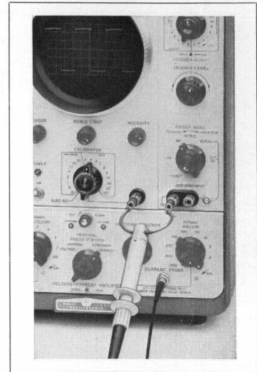
Fig. 11. Amplitude and phase response of probe and amplifier can easily be checked using calibrator on Model 150A Oscilloscope.
