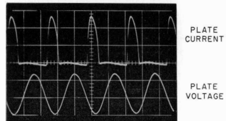
Fig. 2. Oscillogram illustrating type of display obtainable with new probe and plug-in unit. Upper trace shows plate current waveform in an oscillator circuit, while lower trace shows oscillator plate voltage.
