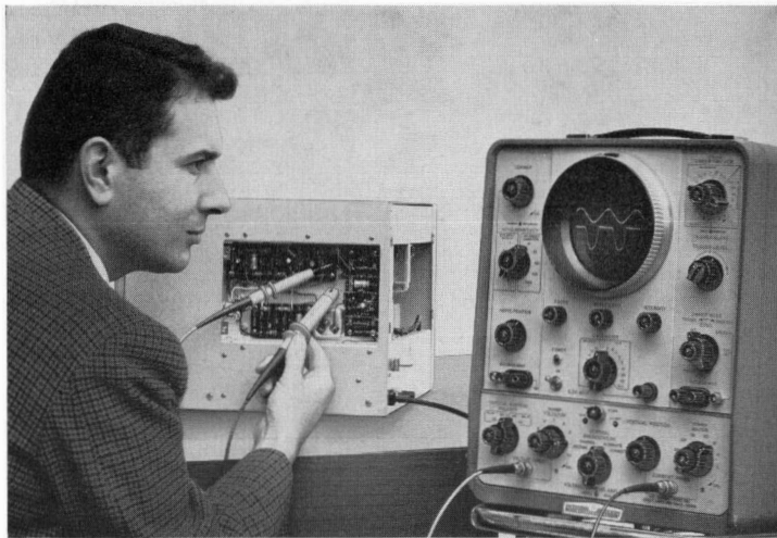
Fig. 1 (at left). New current probe and plug-in unit for Model 150A Oscilloscope enable alternating currents as small as 1 ma and up to 8 mc in frequency to be measured merely by clipping probe on conductor. Unit also includes voltage channel and dual-trace provision to permit voltage to be measured simultaneously with current.
