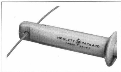
Fig. 4. Current probe clips around conductor to make measurement. Probe jaws are operated by flanges on probe body and accept conductors up to 0.175-inch O.D.
